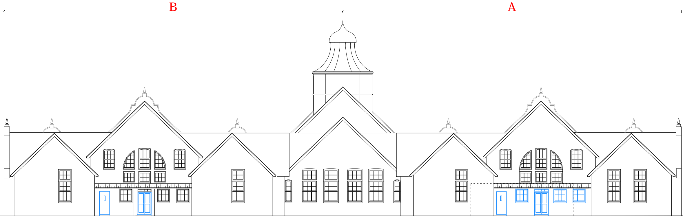
REAR ELEVATION (NO:01 MAIN BUILDING)
